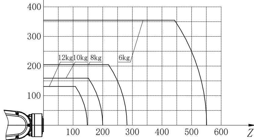
X 负载曲线图 (Load curve)
