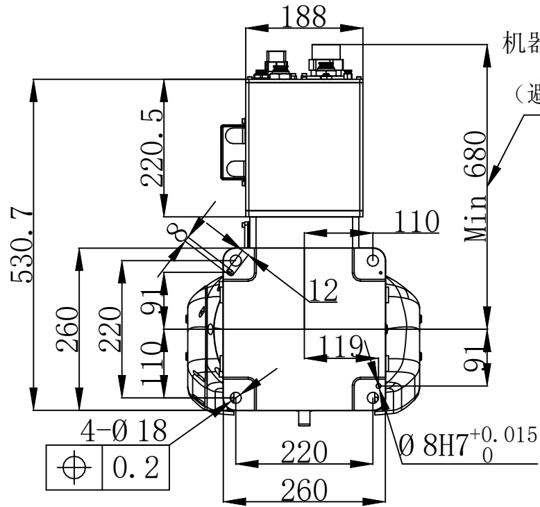
底座安装尺寸图 Installation dimension drawing of base
