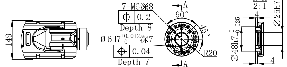
末端法兰安装尺寸图 Installation dimension drawing of end flange 比例 Scale: 2:1
