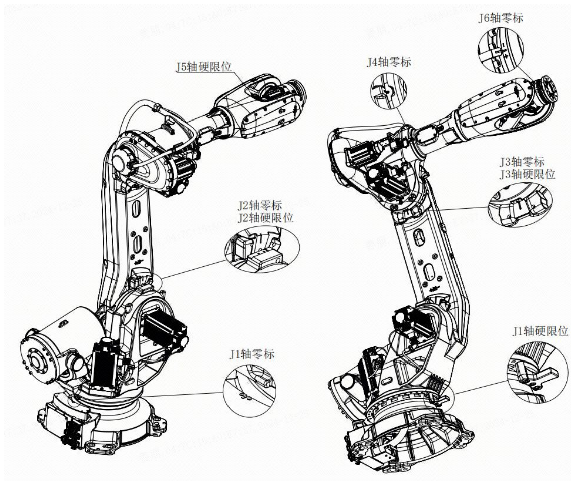
(b) ER230-2700 &amp; ER155-3200
