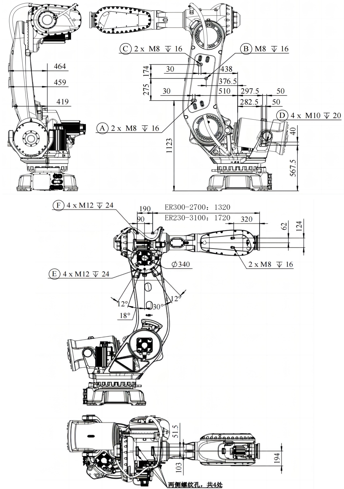
(a) ER300-2700 & ER230-3100
