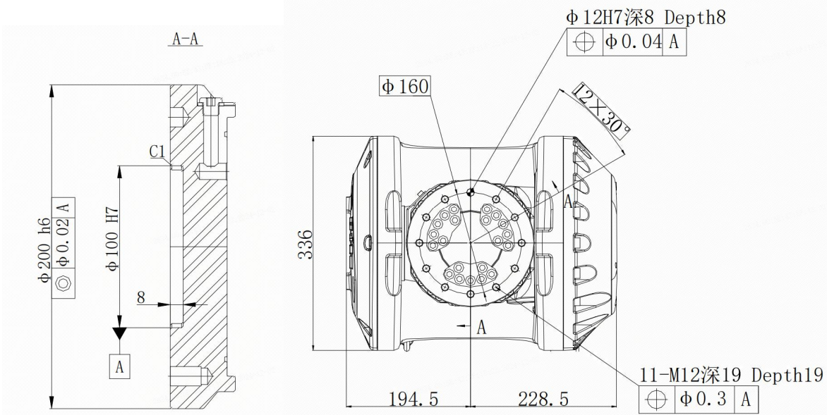
(a) ER300-2700 & ER230-3100
