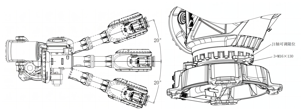
(a) ER300-2700 &amp; ER230-3100
