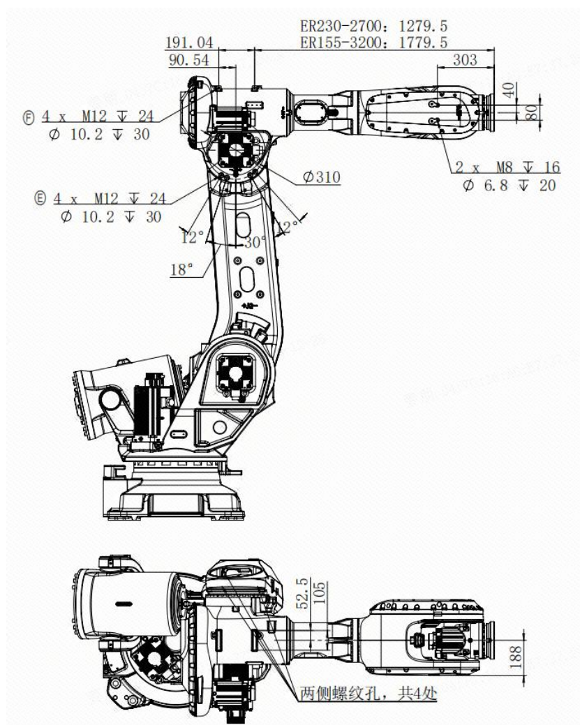
(b) ER230-2700 & ER155-3200
