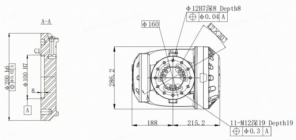
(a) ER230-2700 & ER155-3200
