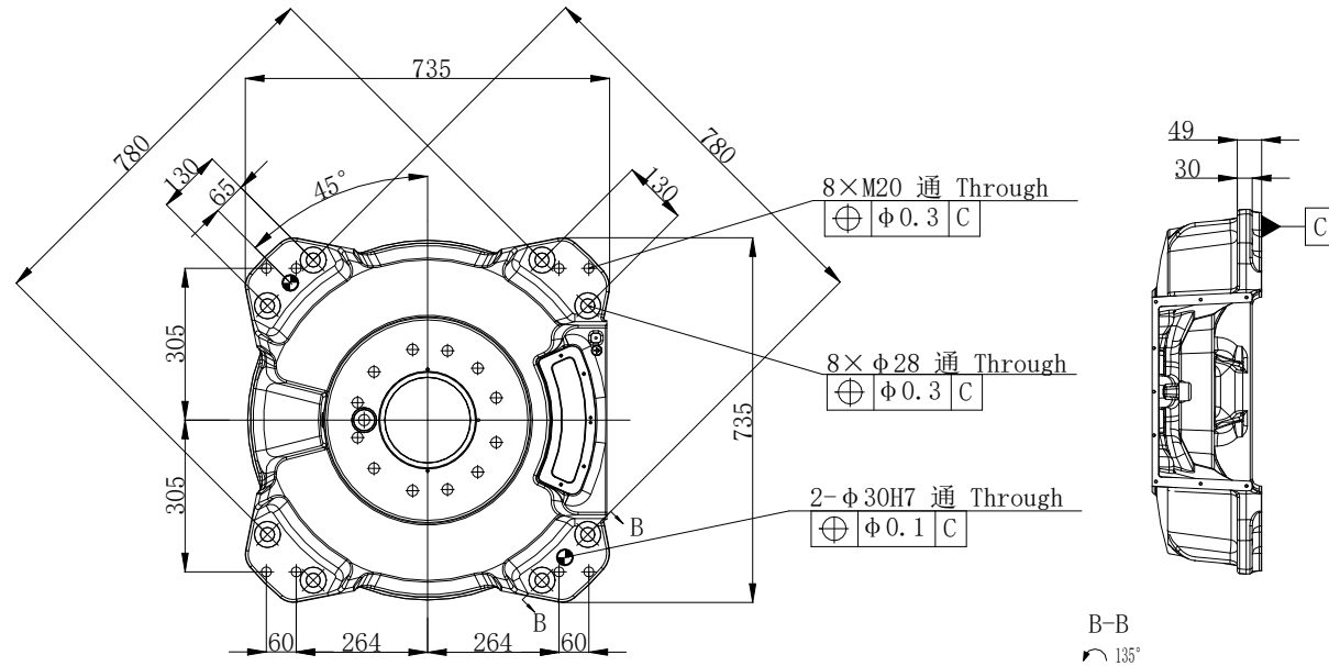
底座安装图(Base mounting size)
