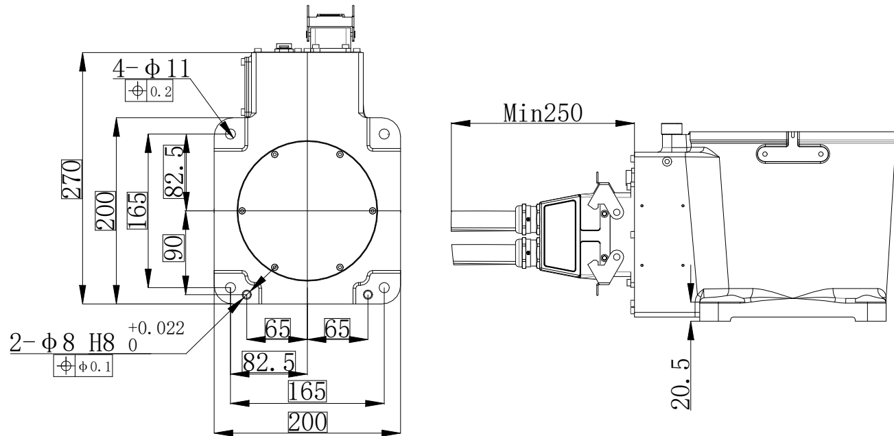
底座安装图(Base mounting size)
