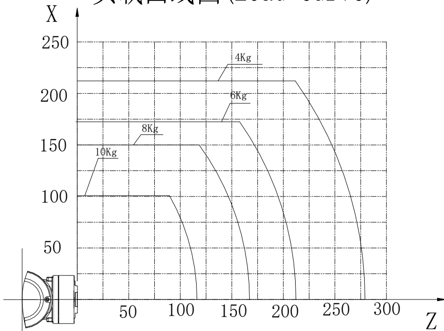
负载曲线图 (Load curve)
