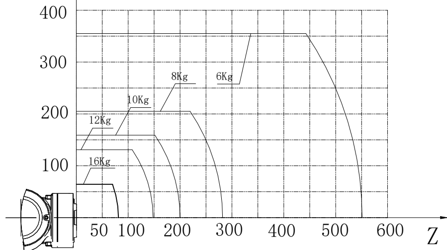
X 负载曲线图 (Load curve)
