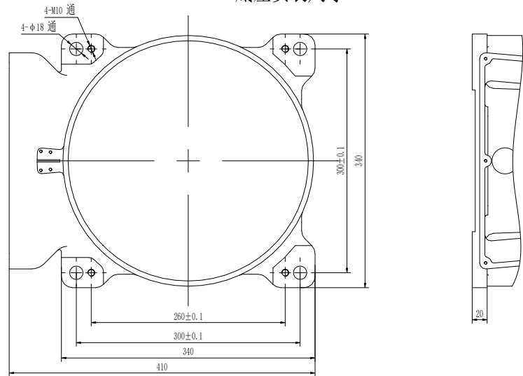
Base mounting size 底座安装尺寸
