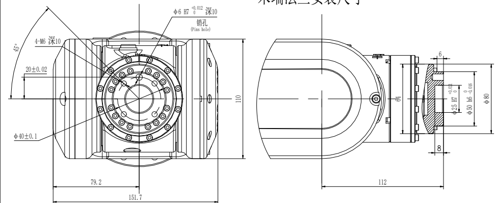
End flange mounting size 末端法兰安装尺寸
