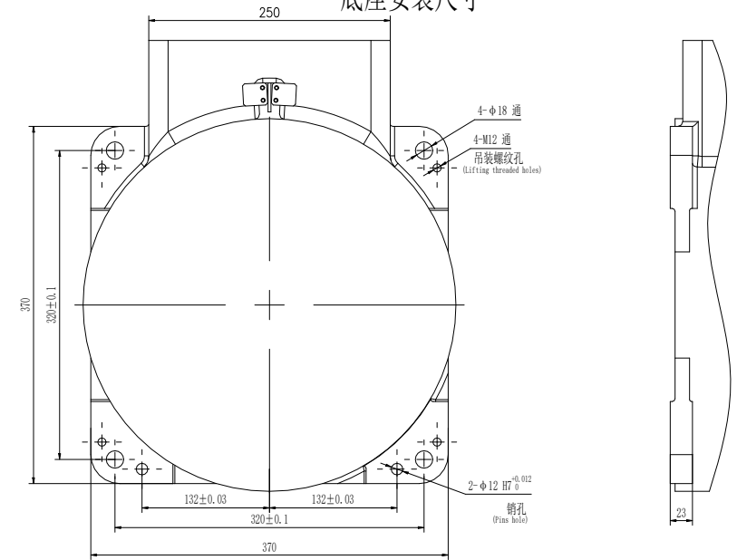
Base mounting size 底座安装尺寸
