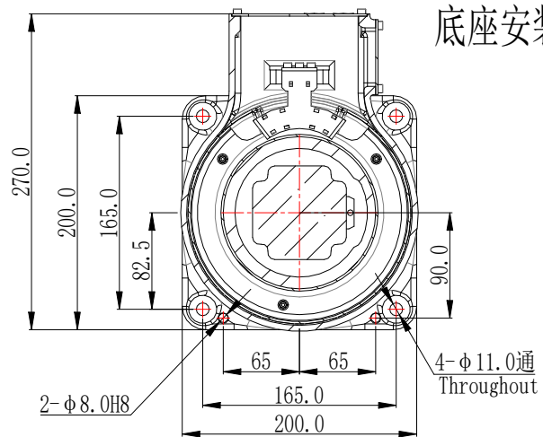
Base mounting diagram
