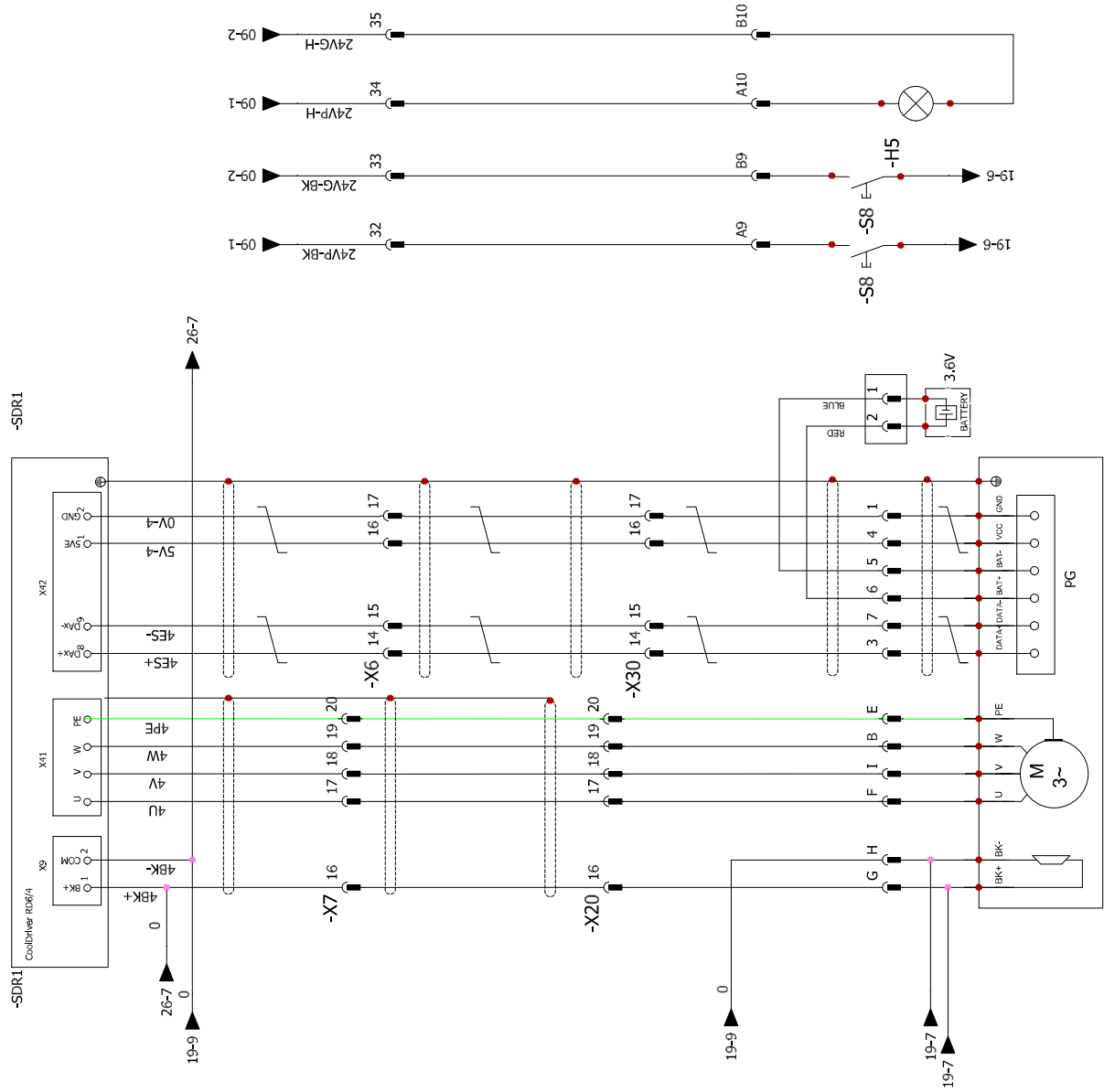
4轴电机动力线、抱闸线、编码器线 4-axis motor power cable, brake cable, encoder cable
