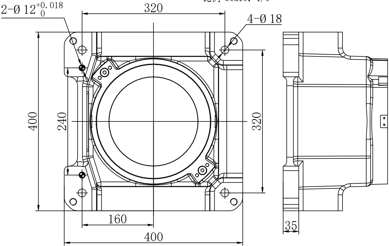
底座安装尺寸图 Installation dimension drawing of base 比例 Scale: 1/5
