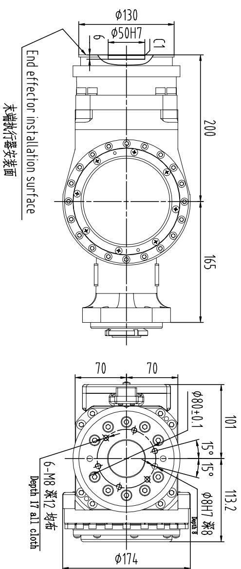
End interface dimension map
